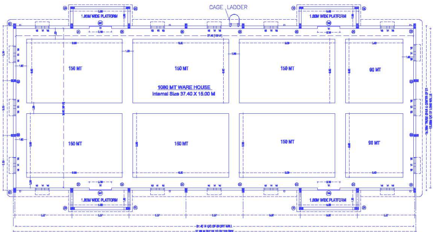
1080 MT WARE HOUSE UNIT PLAN
