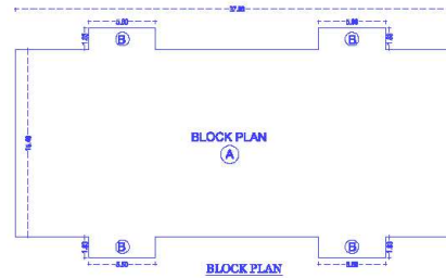
BLOCK PLAN
