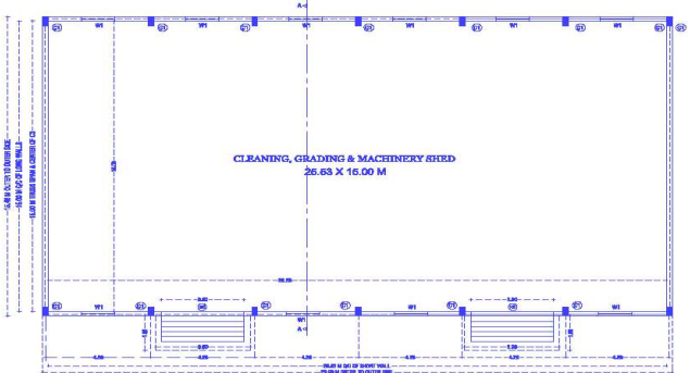
CLEANING ,GRADING & MACHINERY PLANT SHED
